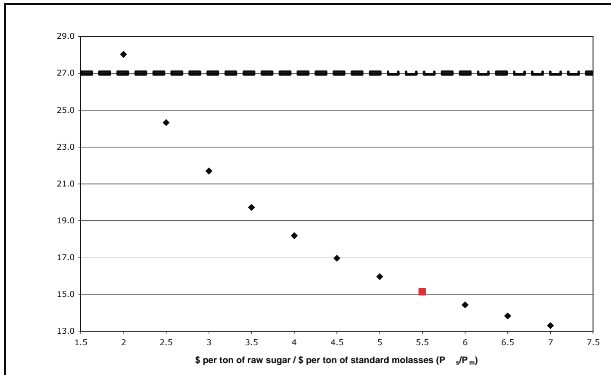
Figure 2. Sensitivity of LCA GHG emissions to the raw sugar to molasses price ratio
