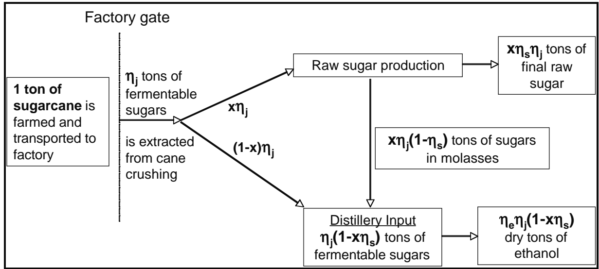
Figure 1. Mass and Process flow of an integrated sugar and ethanol factory
